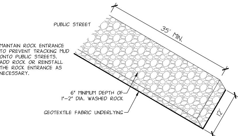
ROCK CONSTRUCTION ENTRANCE
