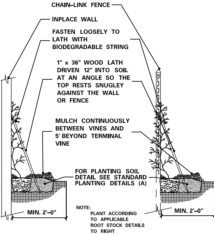
WALL INSTALLATION
